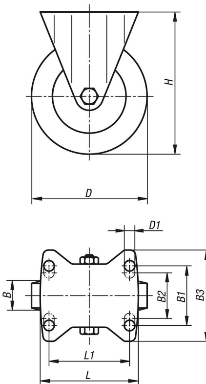
fixed castor
